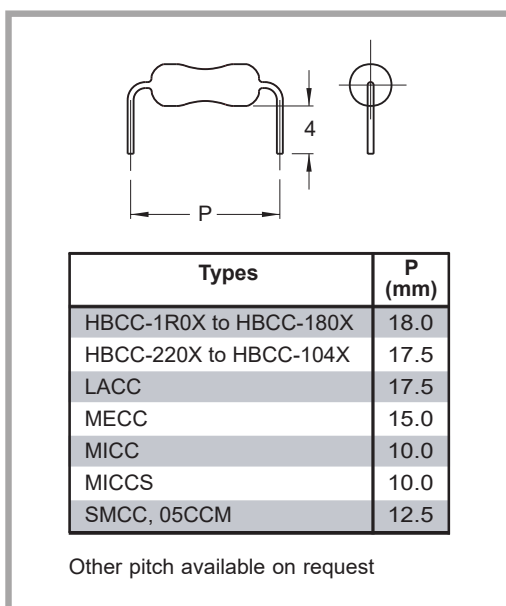
Fig. 7: Axial preformed
